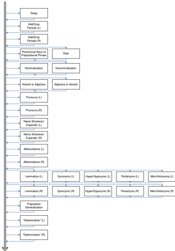
Figure 2. Diagram of pathways through the BE transformation pipeline. 'L' and 'R' indicate whether the transformation is limited to the left-most or rightmost word in the BE.
