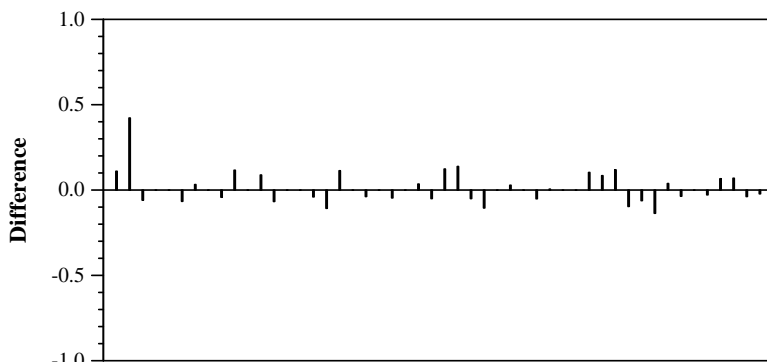
Question Difference from median for squishy list F score ( \beta = 3 )
