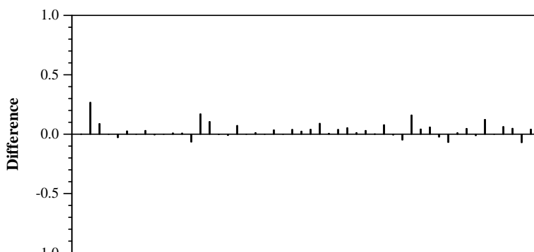
Series Difference from median for per-series combined score
