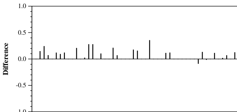
Question Difference from median for rigid list F score
